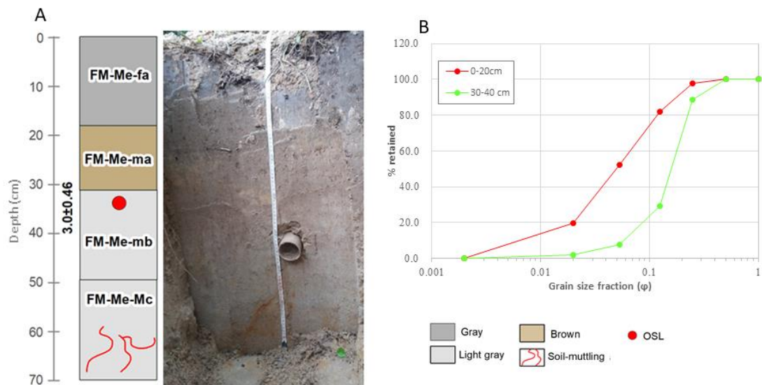
Figure 4. Surficial cover deposit of the fluvial-marine terrace on the left bank. A) Allostratigraphic profile. B) Grain-size curves. FM: Fluvial-marine. Me: left bank. fa: Fluvial depositional processes. ma to me: Marine depositional processes.
